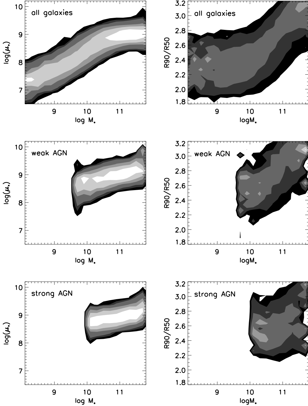
Figure 9: Left: Conditional density distributions showing trends in the surface mass density \mu_* as a function of stellar mass M_* for all galaxies (top), for weak AGN with \log L[\text{OIII}] < 7.0 (middle) and for strong AGN with \log L[\text{OIII}] > 7.0 (bottom). Each object has been weighted by 1/V_{max} and the bivariate distribution has been normalized to a fixed number of galaxies in each bin of \log M_* . Right: Conditional density distributions showing trends in concentration index C as a function of \log M_* . In this and all other conditional density plots, each contour represents a factor 2 increase in density.
